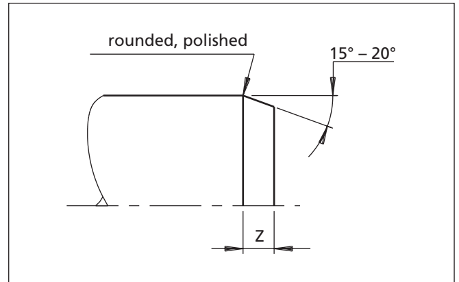
Figure 12 Lead-in chamfer for rods, shafts
