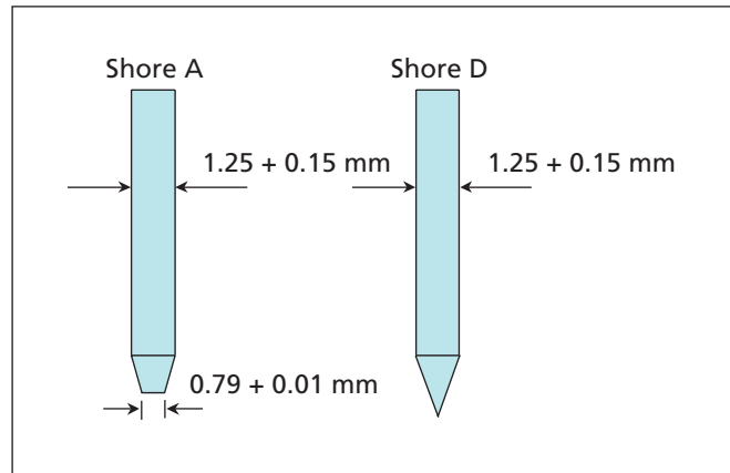
Figure 3 Indentor according to Shore A / D
