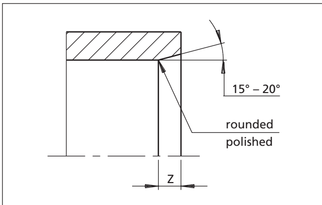
Figure 11 Lead-in chamfer for bores, tubes
