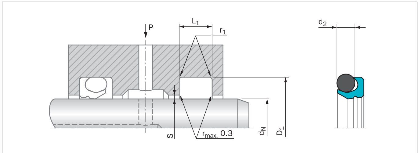
Figure 150: 安装图纸
