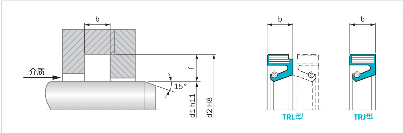
Figure 45: 安装图纸
