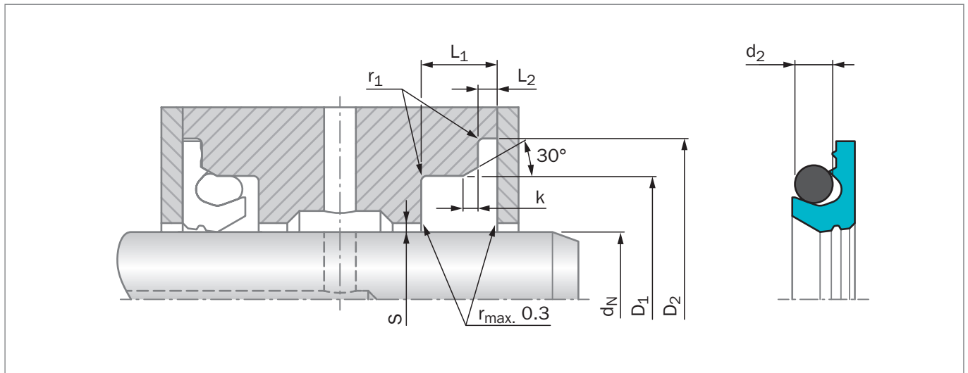
Figure 145: 安装图纸
