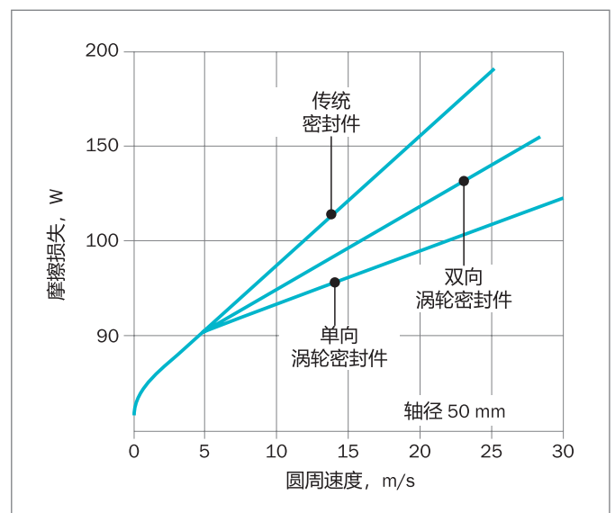
Figure 32: 摩擦损失
