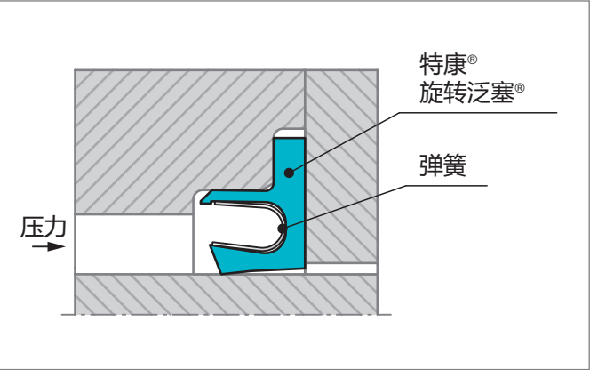
Figure 138 特康®旋转泛塞®
