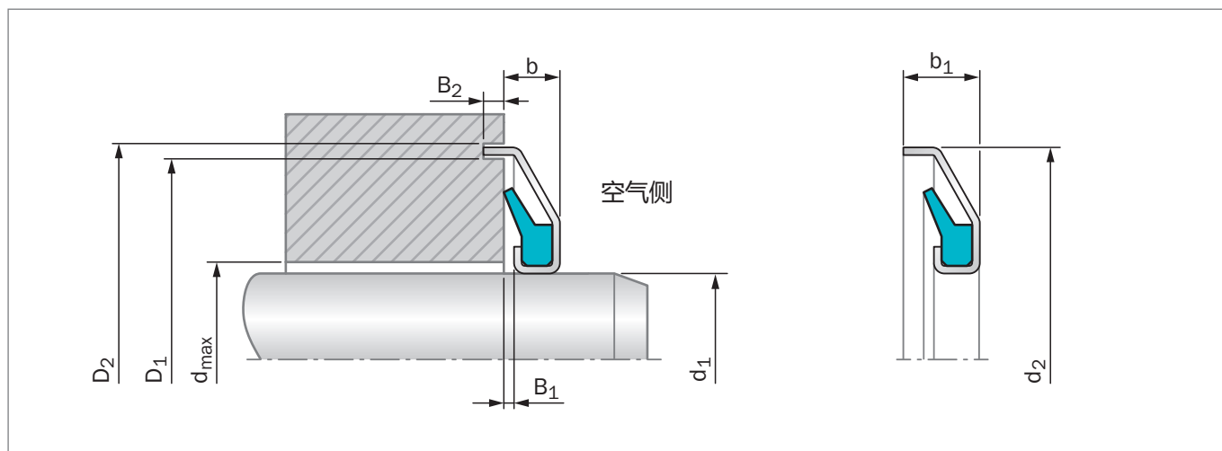
Figure 90: GAMMA密封件，带迷宫
