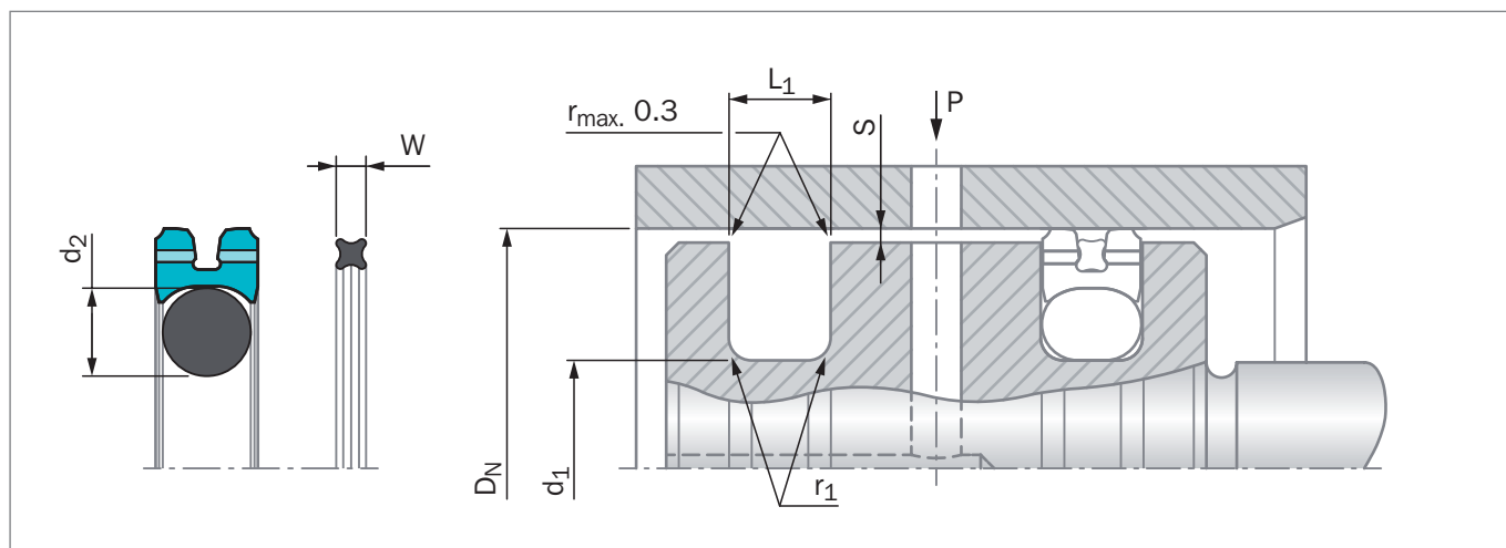
Figure 132 安装图纸
