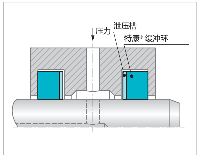
Figure 169: 特康®缓冲环的正确安装
