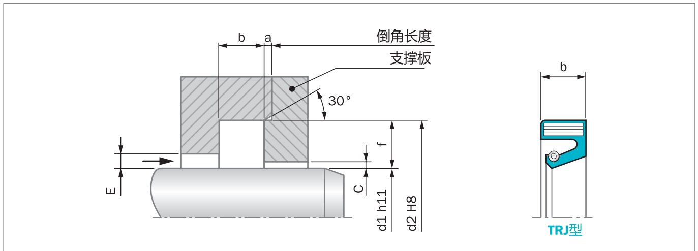
Figure 43: 安装图纸
