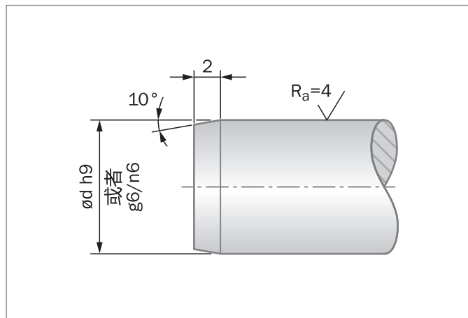
Figure 85: 轴的公差、表面粗糙度和轴的倒角
