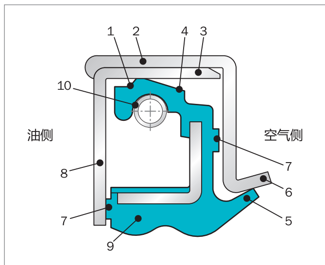
Figure 46: 系统500
