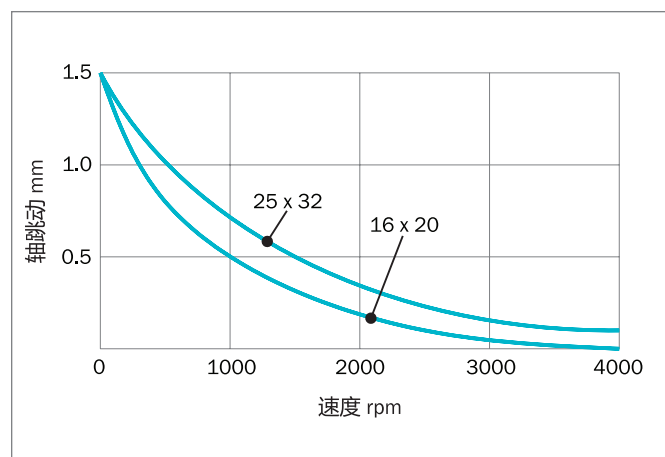
Figure 42: 轴跳动
