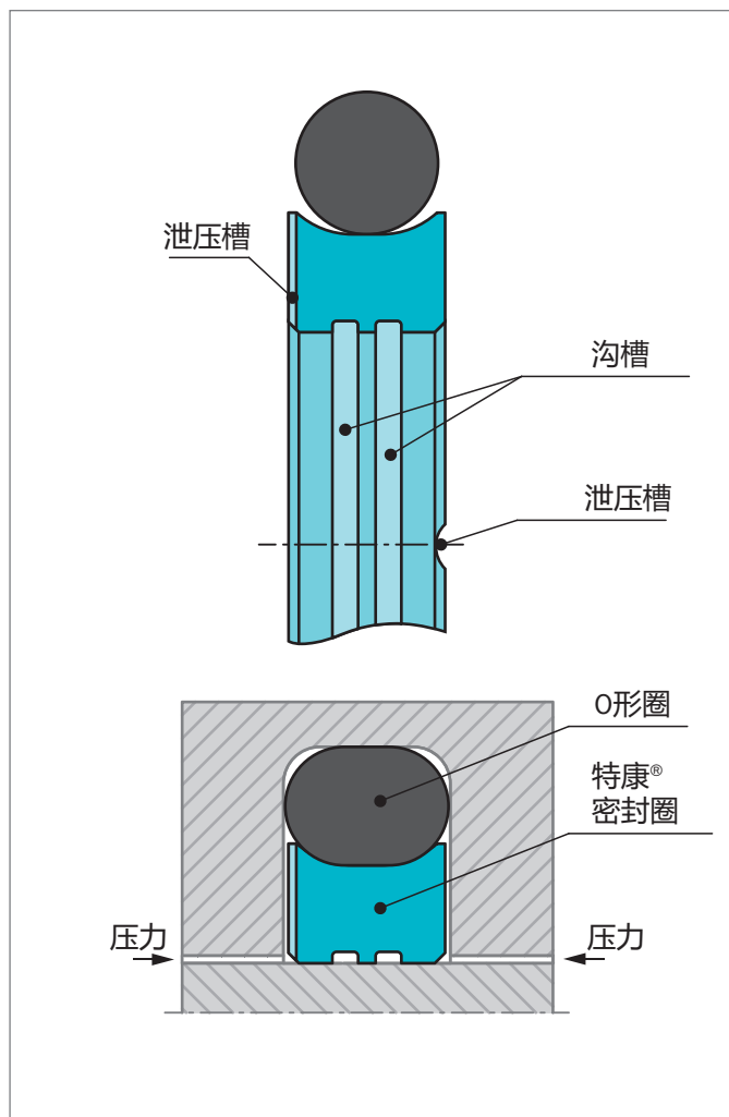
Figure 117: 特康®旋转格来圈®
