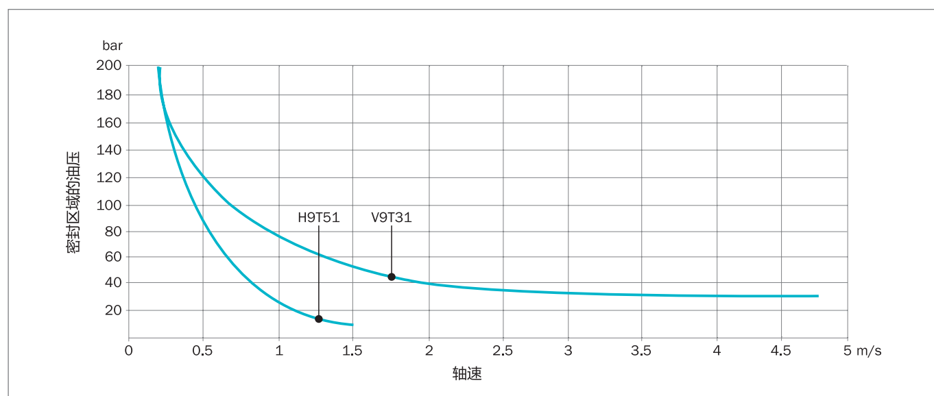
Figure 25: HP20额定工况
