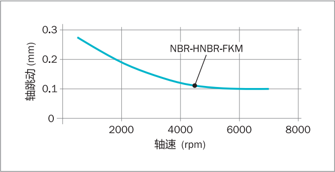
Figure 56: 允许的轴跳动
