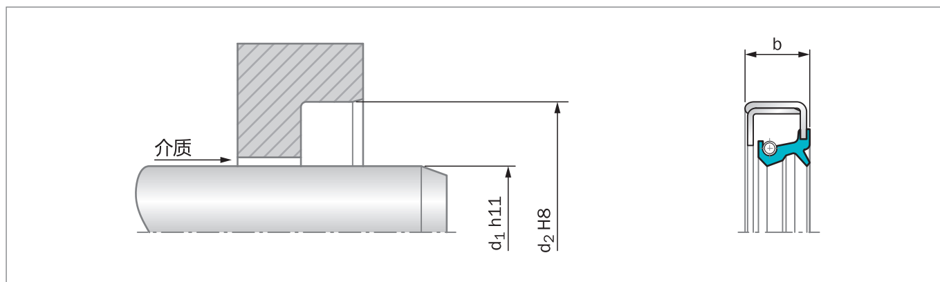
Figure 19: 安装图纸
