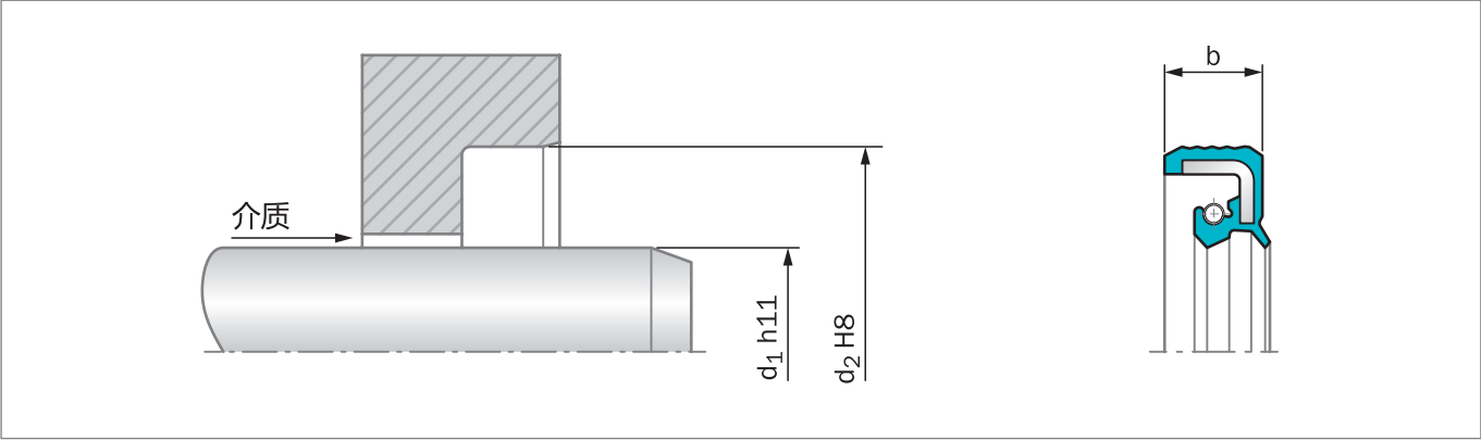
Figure 22: 安装图纸
