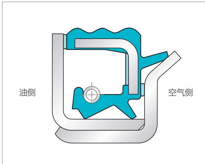
Figure 50: 系统5000
