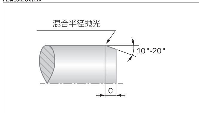
Figure 140 轴的引入倒角
