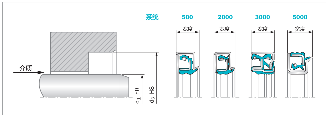
Figure 52: 安装图纸
