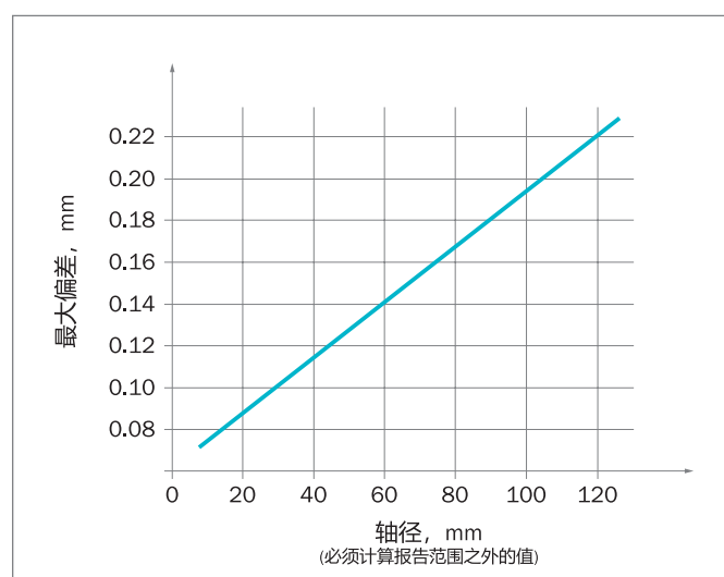
Figure 26: 轴孔偏差
