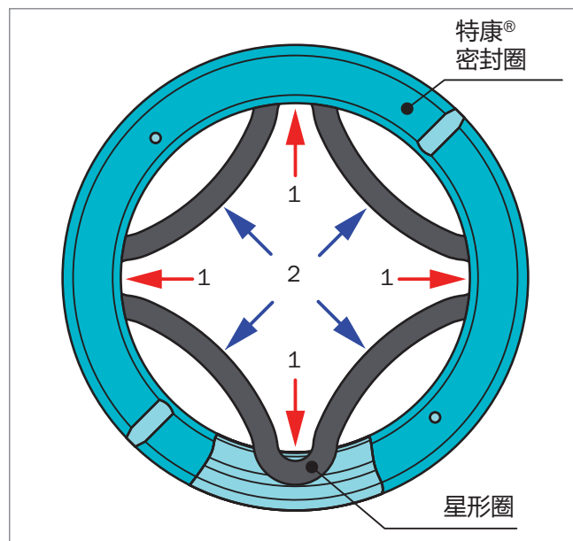
Figure 159: 斜着插入星形圈的各段进入润滑沟槽
