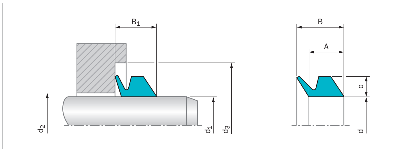
Figure 77: 安装图纸
