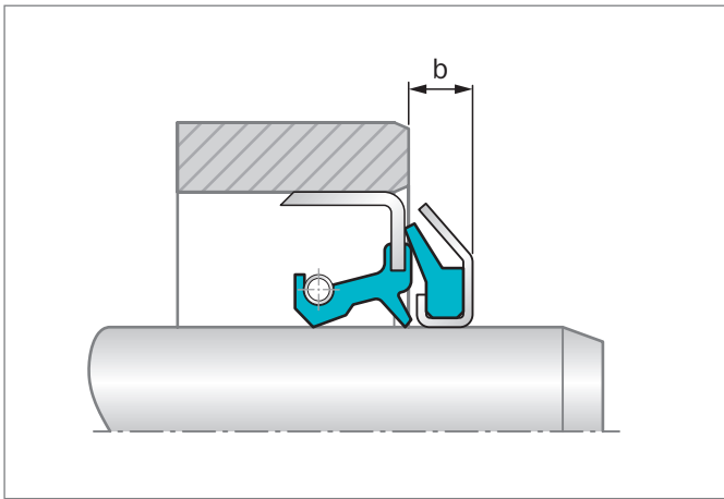
Figure 33: GAMMA seal装配在轴端
