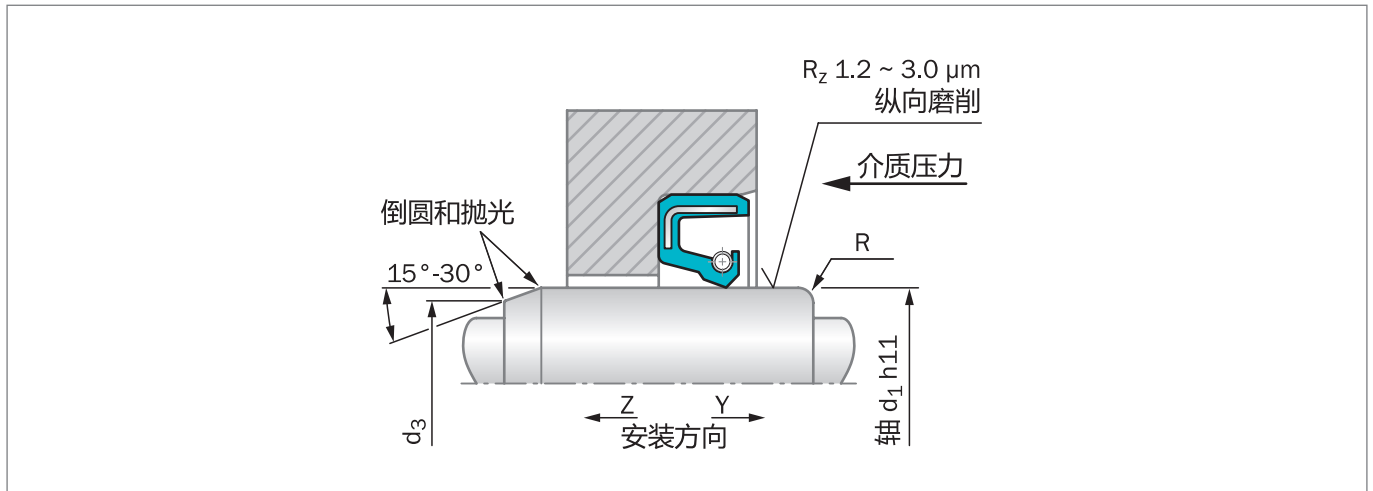
Figure 4: 径向油封的安装
