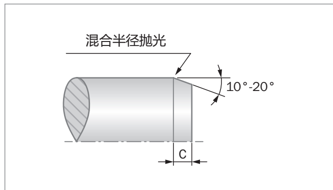
Figure 166: 轴的引入倒角
