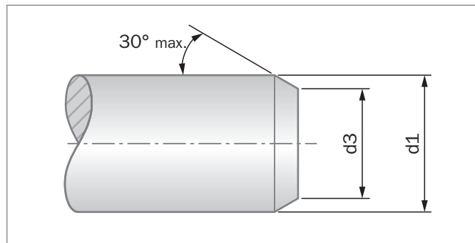
Figure 109: 轴引入倒角
