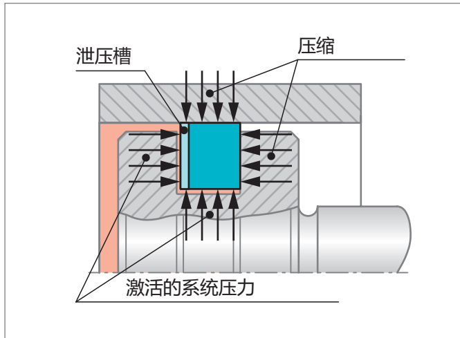
Figure 168: 特康®缓冲环的压力激活
