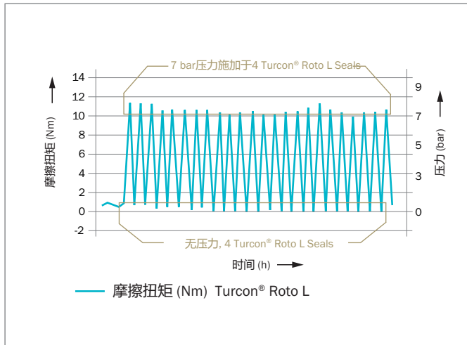
Figure 93: 干气扭矩测试
