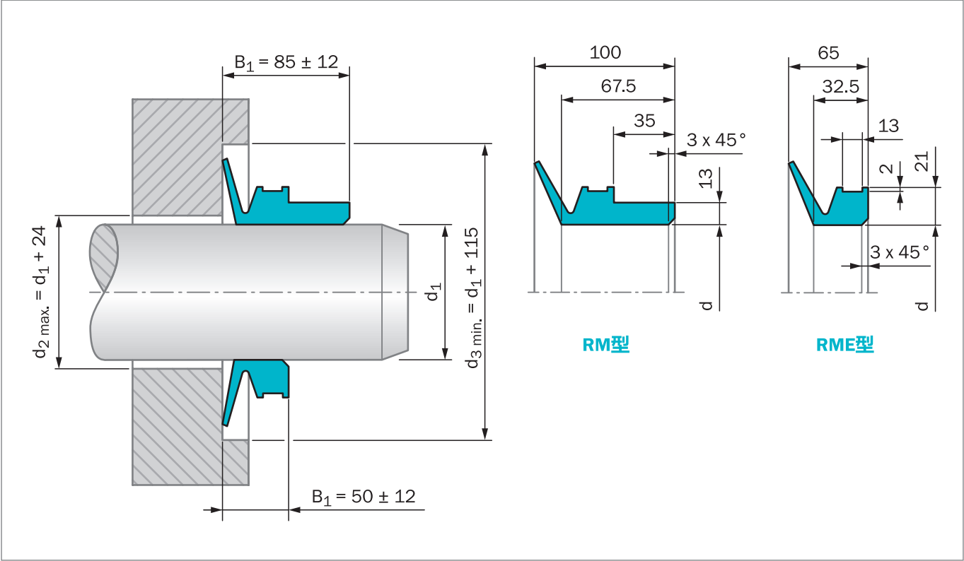
Figure 79: 安装图纸
