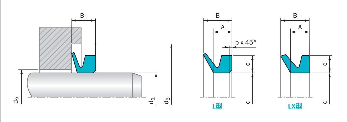
Figure 78: 安装图纸
