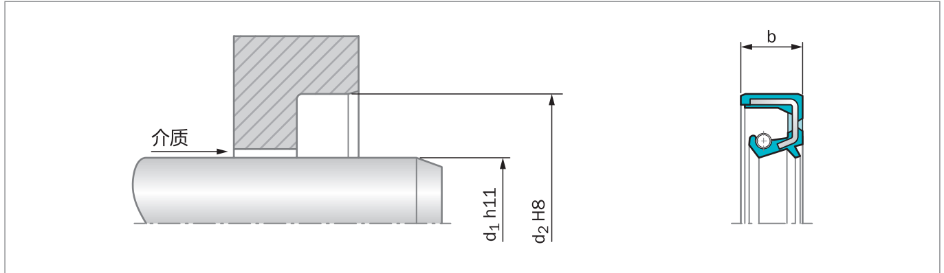
Figure 21: 安装图纸
