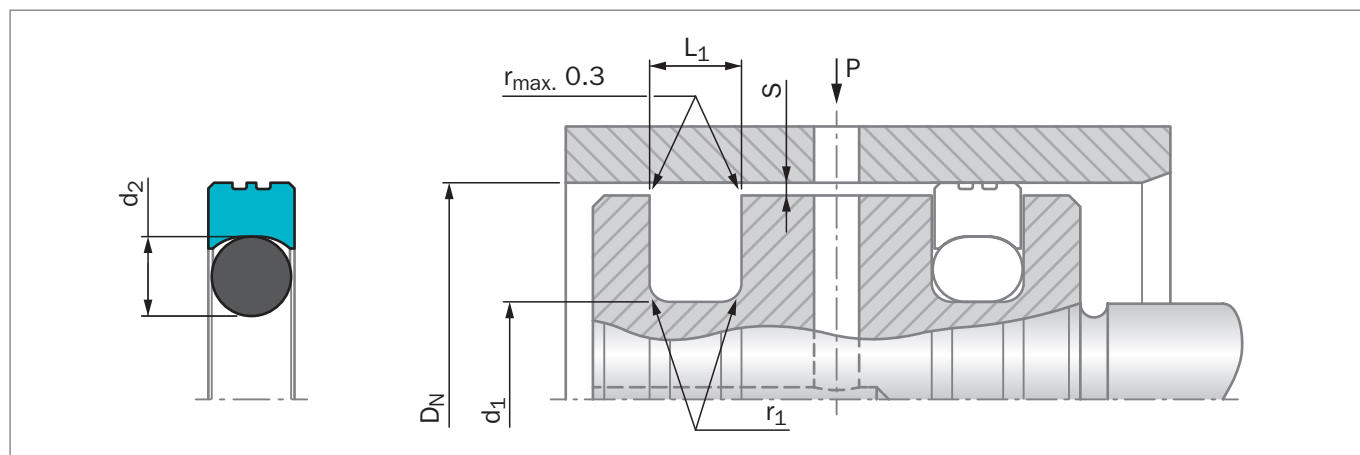
Figure 121: 安装图纸
