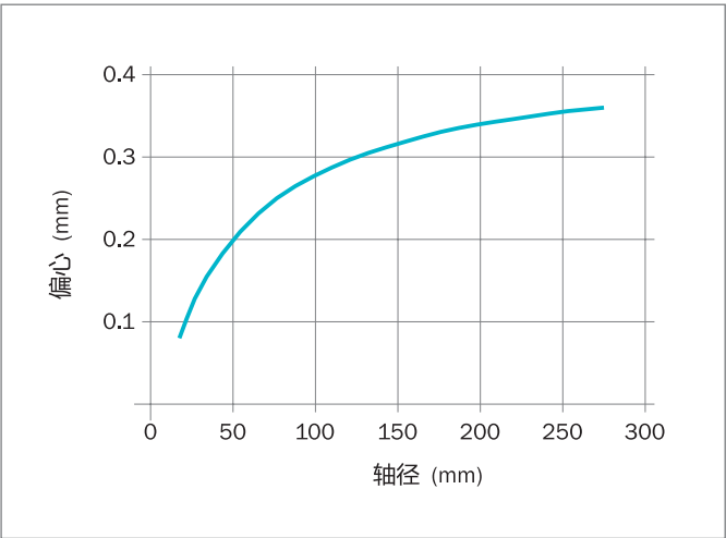
Figure 57: 允许的轴偏心
