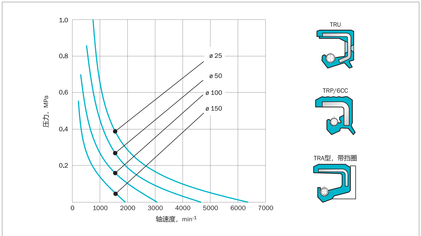
Figure 9: 允许的过压，针对带支撑唇的密封件和针对受压密封件
