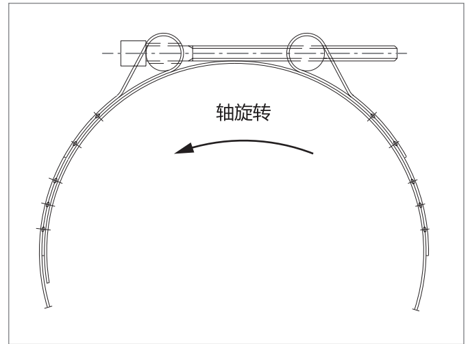
Figure 74: 夹紧箍RM
