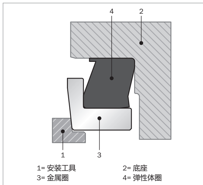
Figure 184: DF型安装工具
