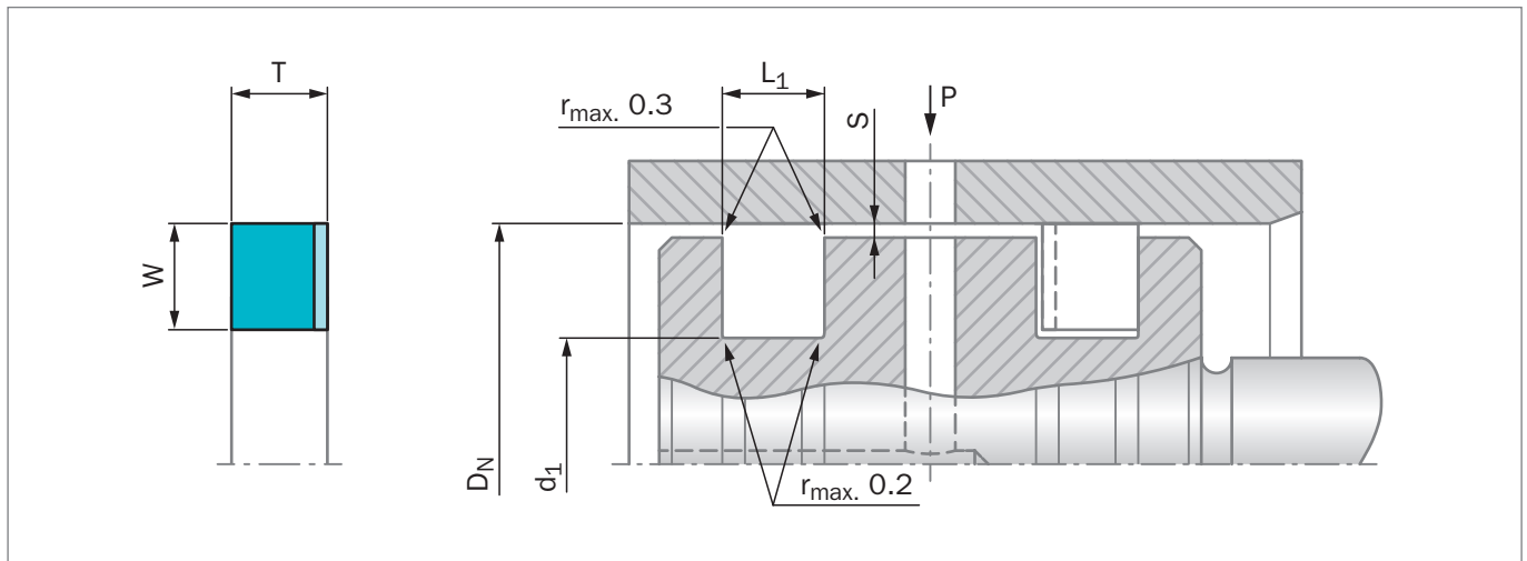
Figure 172: 安装图纸
