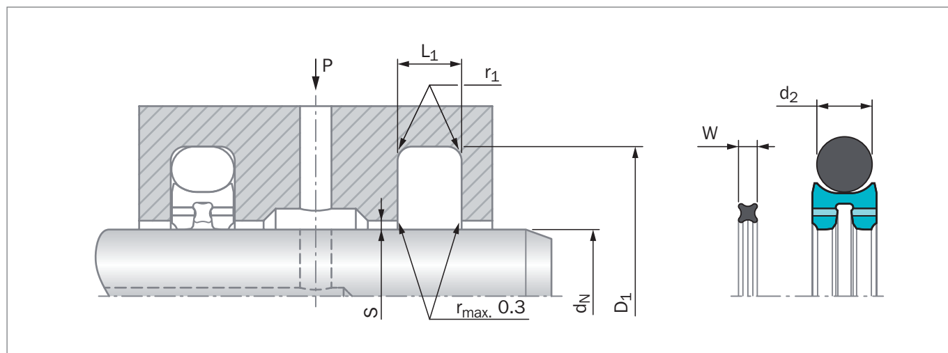
Figure 131 安装图纸
