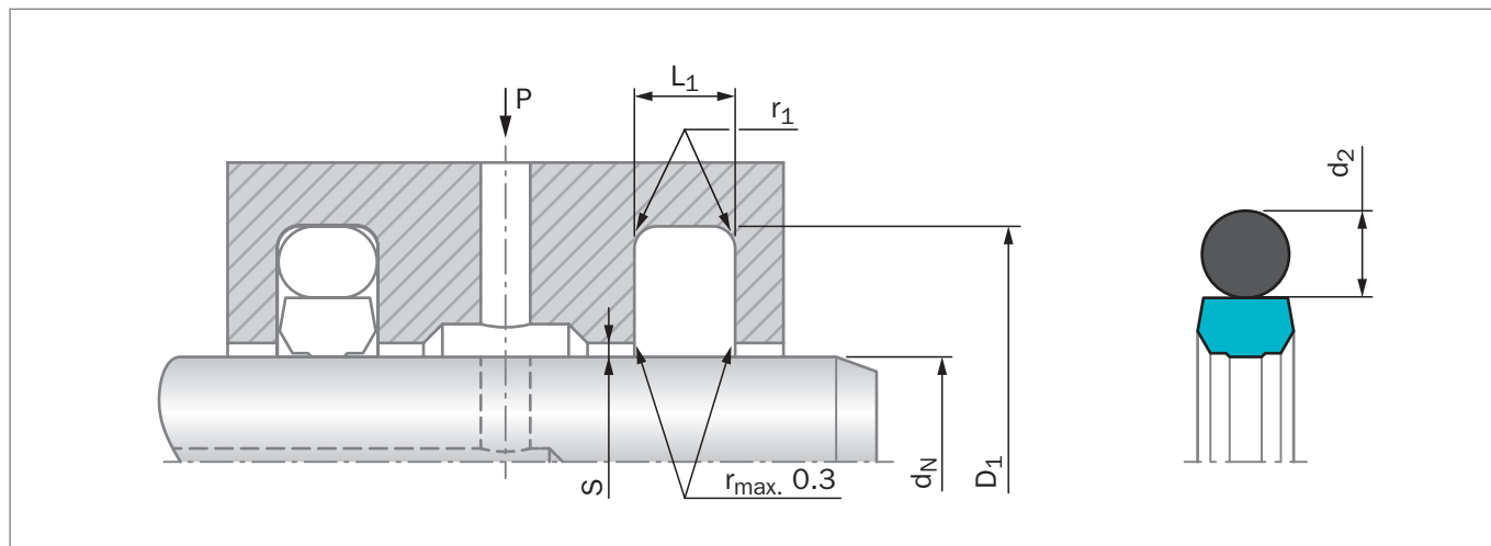
Figure 136 安装图纸
