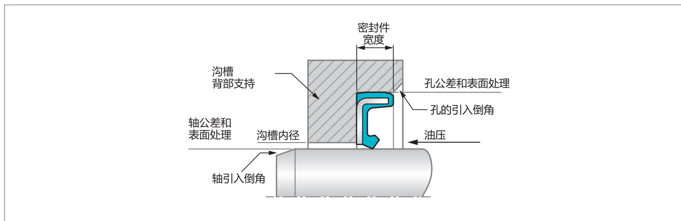
Figure 27: 安装图纸
