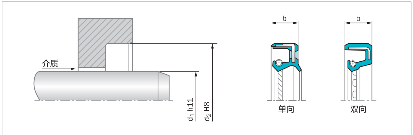
Figure 31: 安装图纸
