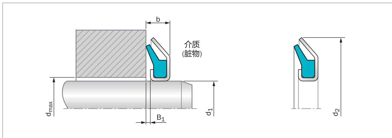
Figure 89: 安装图纸
