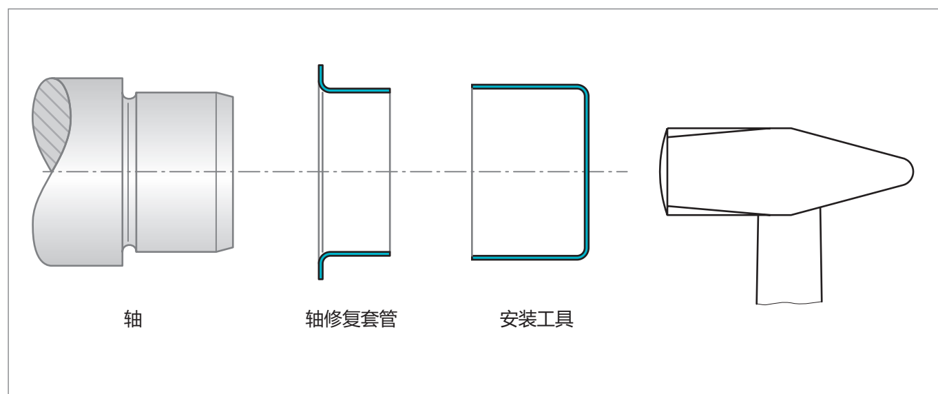
Figure 67: 安装顺序
