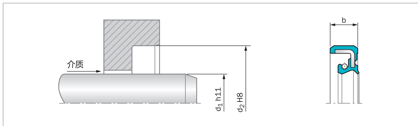
Figure 23: 安装图纸
