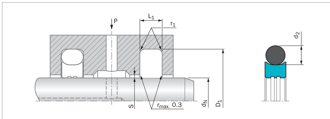
Figure 120: 安装图纸
