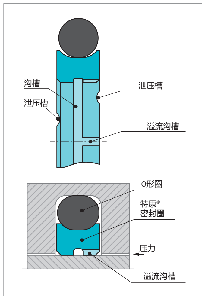
Figure 122: 带泄压功能的特康®旋转格来圈®K
