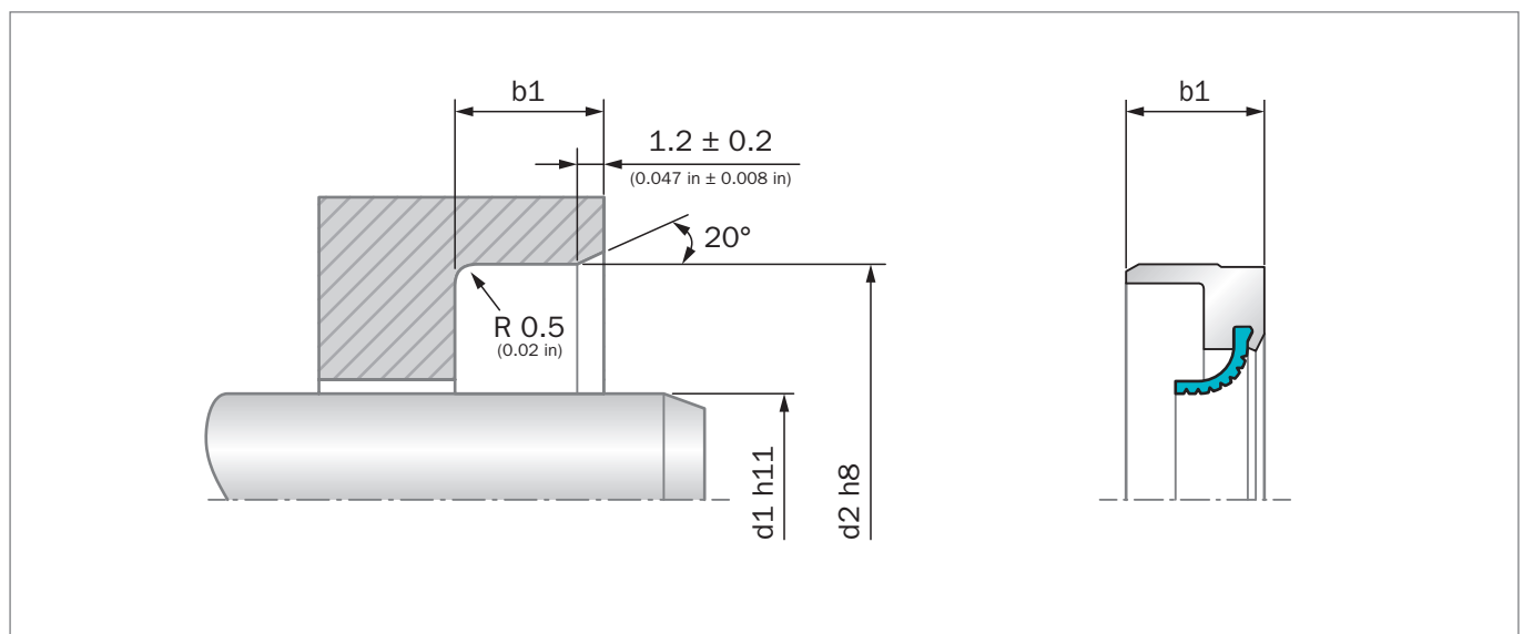
Figure 113: 压力高达0.5 MPa (73 psi)的安装图纸
