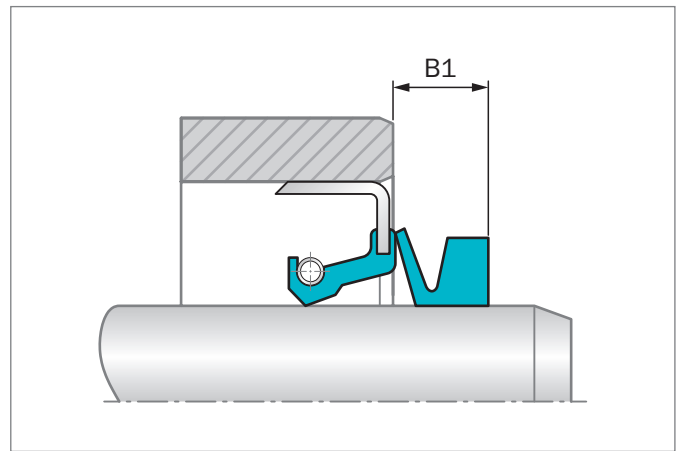
Figure 35: V形圈装配在轴端
