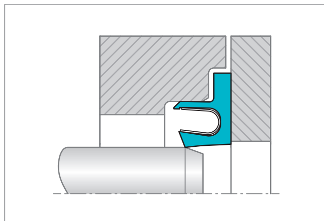
Figure 141 特康®旋转泛塞®
