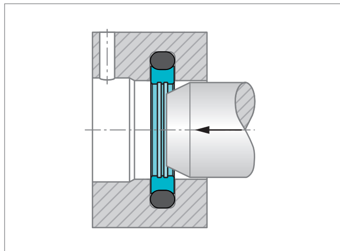
Figure 158: 旋转格来圈®安装后的校准
