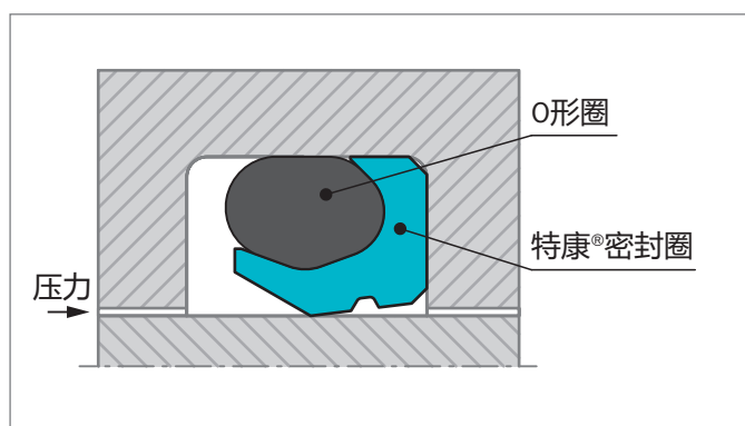
Figure 147: 特康®旋转VL Seal®
