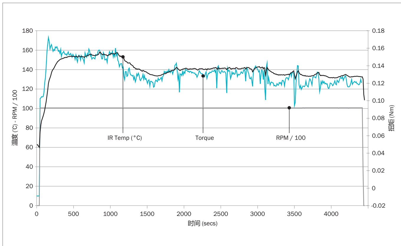
Figure 102: 特康®泛力®PDR密封件的运行扭矩
