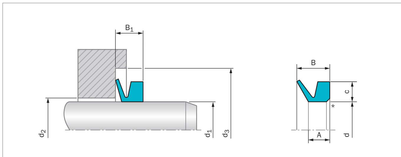
Figure 76: 安装图纸
