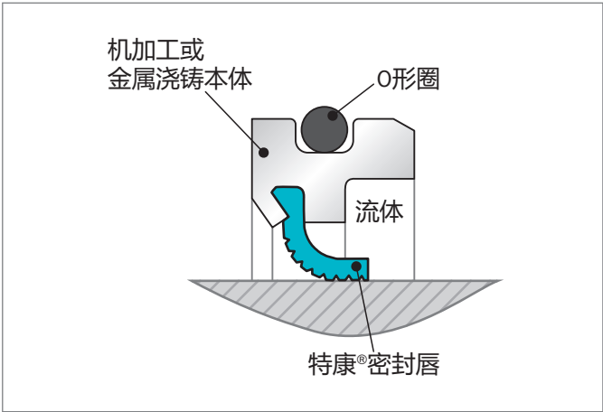
Figure 97: O形圈设计
