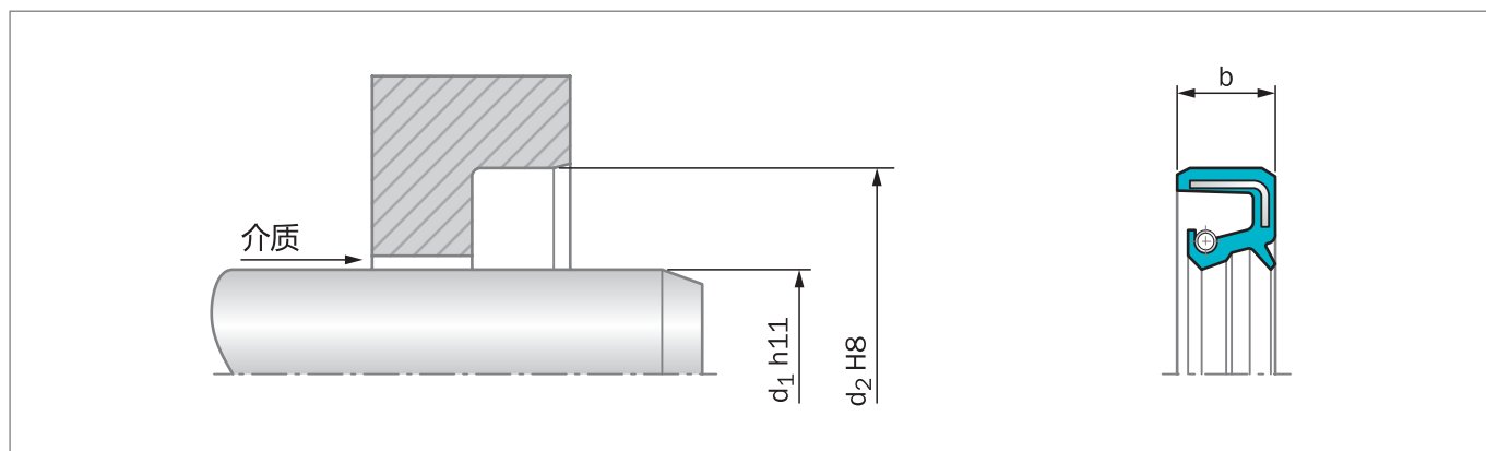
Figure 15: 安装图纸
