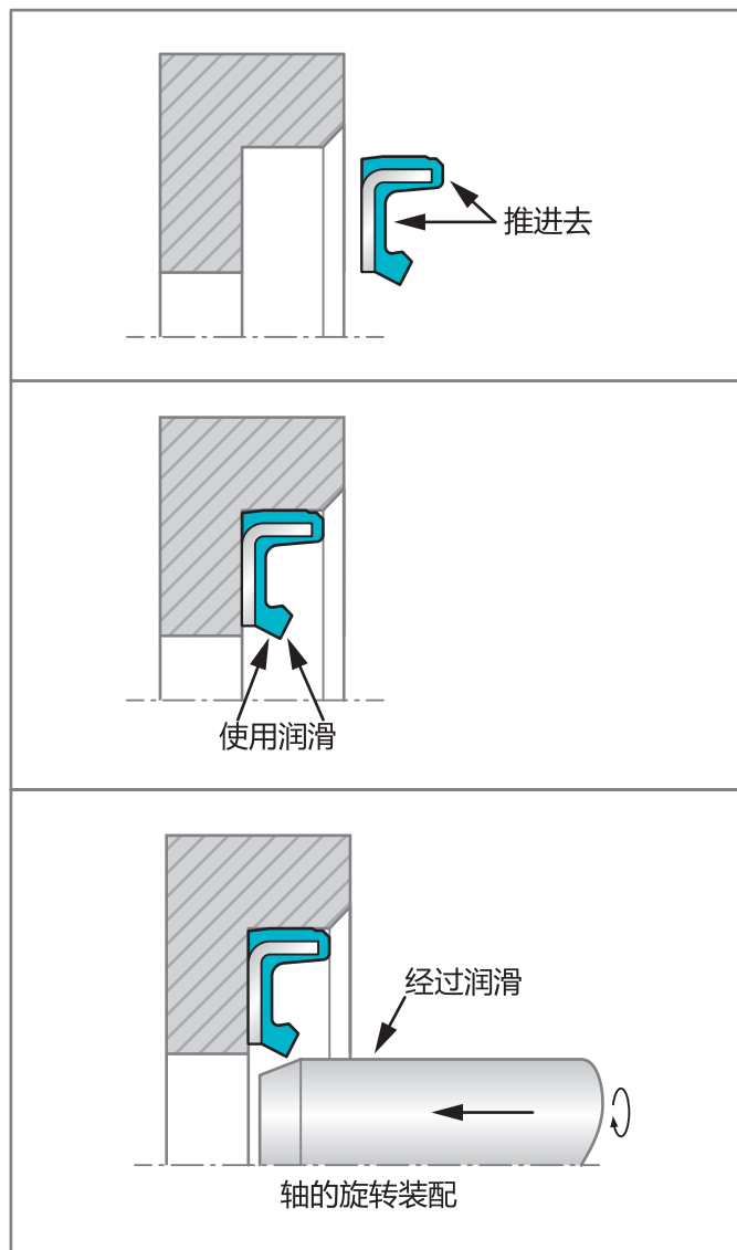
Figure 28: 安装指导
