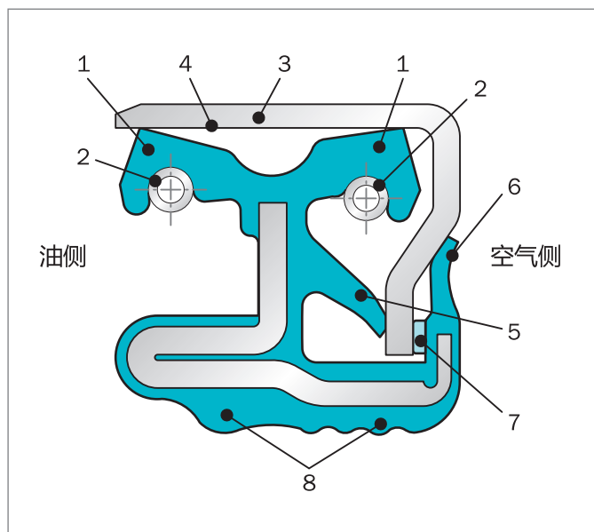
Figure 48: 系统3000
