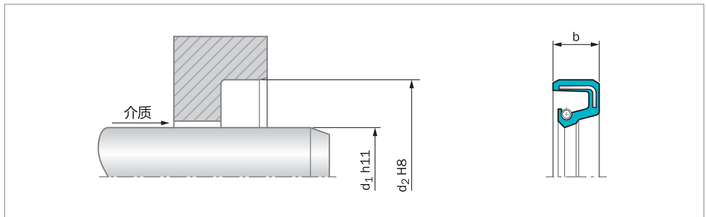
Figure 14: 安装图纸
