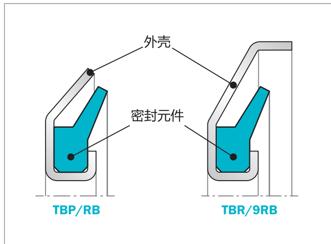
Figure 81: GAMMA密封件
