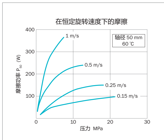
Figure 139 ®特康®旋转泛塞®的摩擦功率
