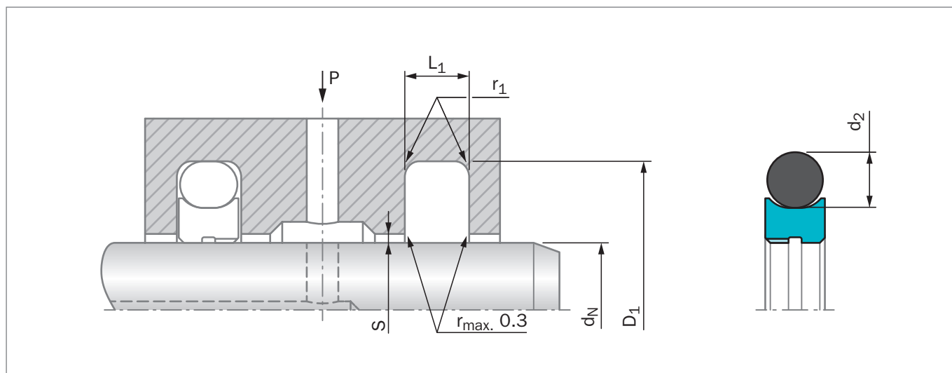
Figure 125: 安装图纸
