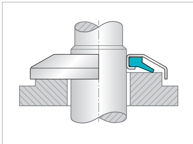
Figure 83: 垂直安装
