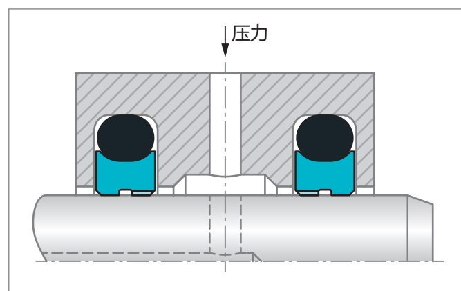
Figure 123: 旋转格来圈®K的正确安装
