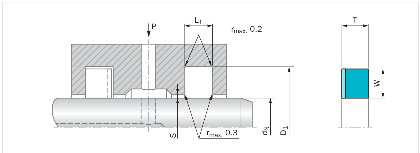
Figure 171: 安装图纸
