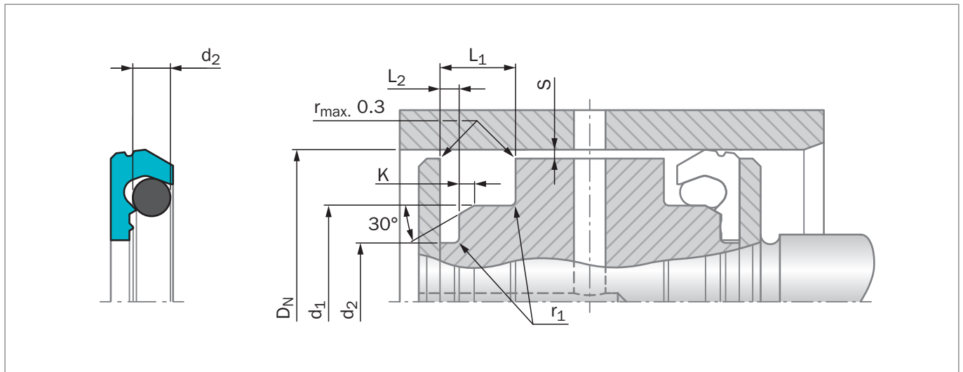
Figure 146: 安装图纸
