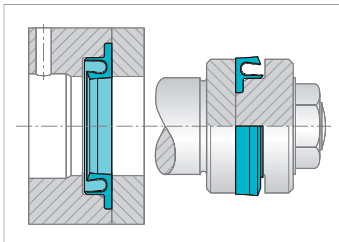
Figure 154: 旋转泛塞®安装
