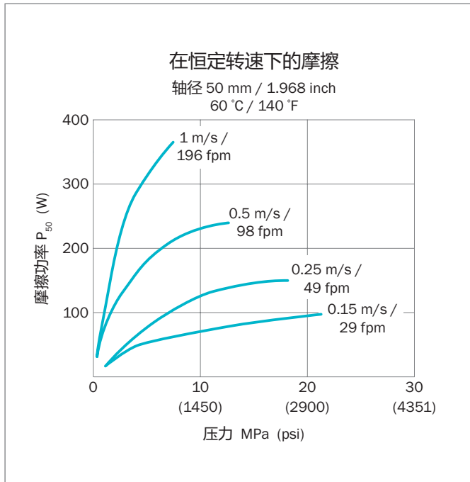
Figure 149: 特康®旋转VL Seal®的摩擦功率
