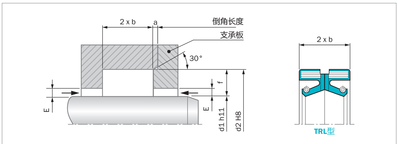
Figure 44: 安装图纸
