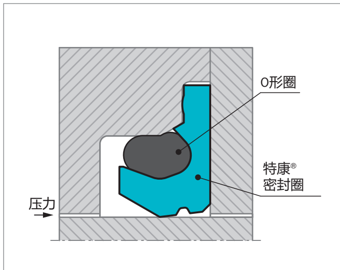
Figure 143: 特康®旋转VL Seal®F
