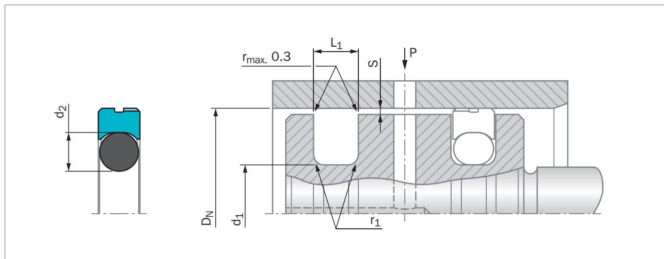
Figure 126: 安装图纸
