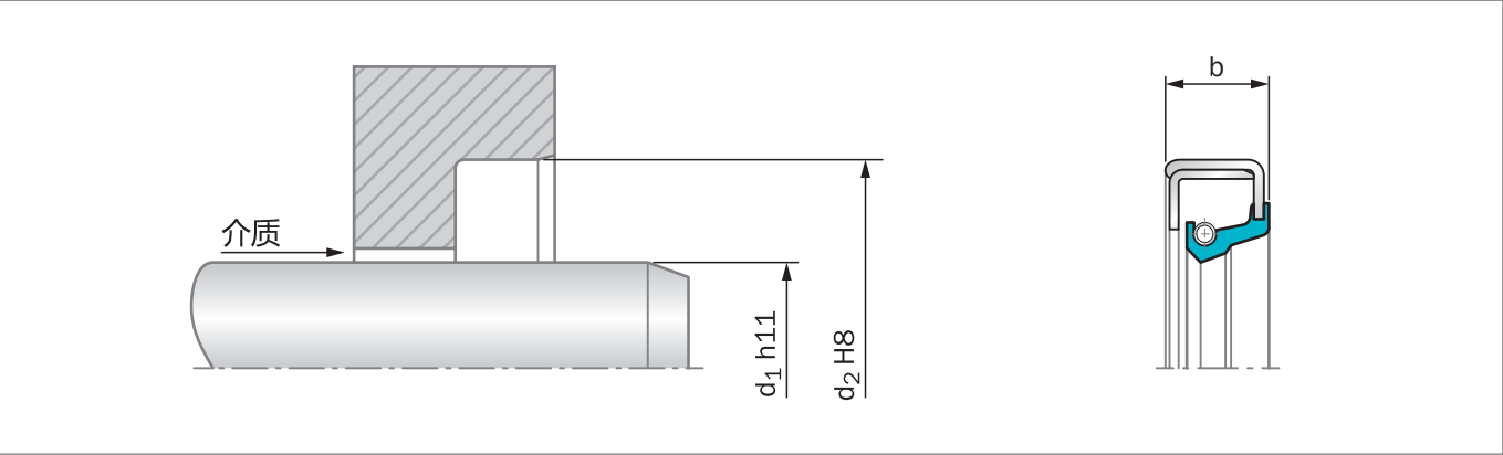
Figure 18: 安装图纸
