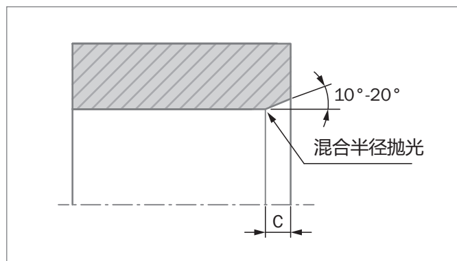
Figure 167: 缸孔的引入倒角
