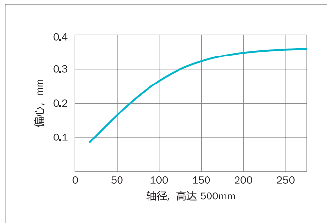
Figure 3: 偏心
