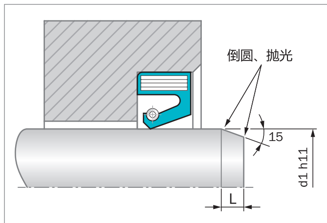
Figure 40: 油封的安装
