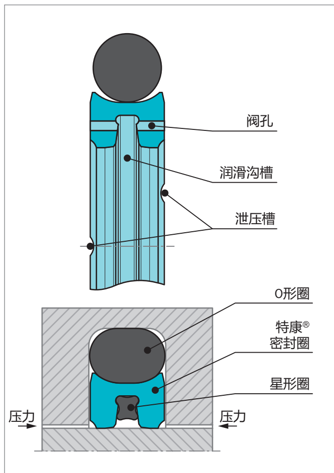
Figure 127 带泄压功能的特康®旋转格来圈®V
