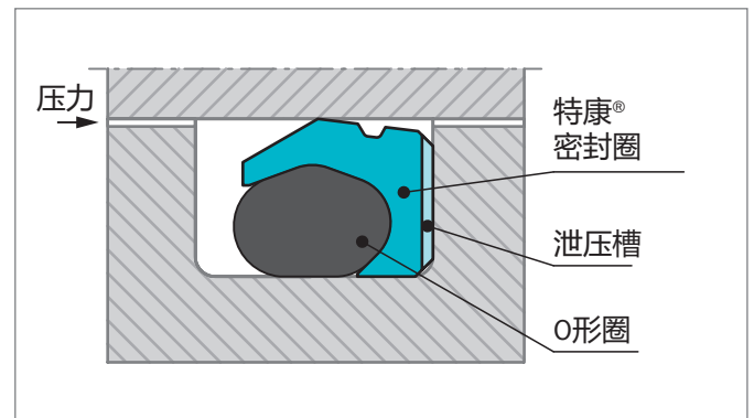
Figure 148: 带径向泄压槽的特康®旋转 VL Seal®
