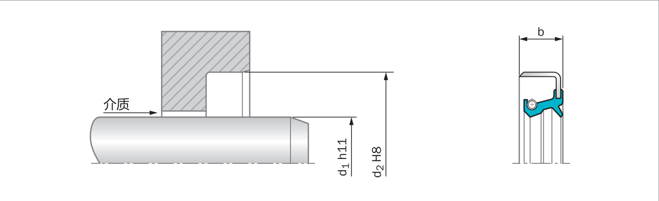
Figure 17: 安装图纸
