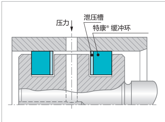
Figure 170: 特康®缓冲环的正确安装
