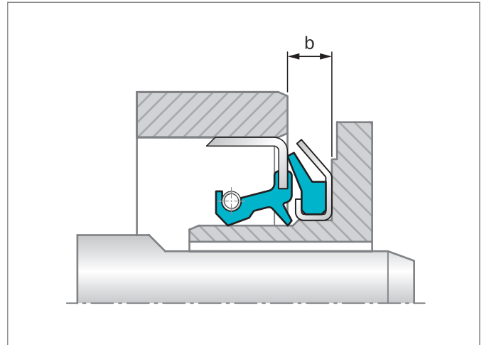
Figure 34: GAMMA seal装配在轴套
