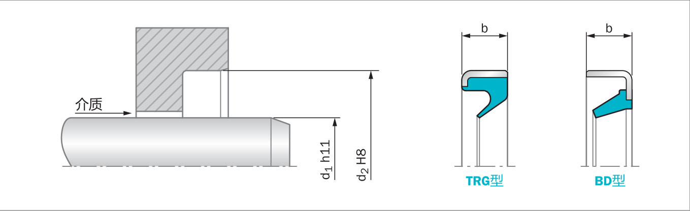
Figure 30: 安装图纸
