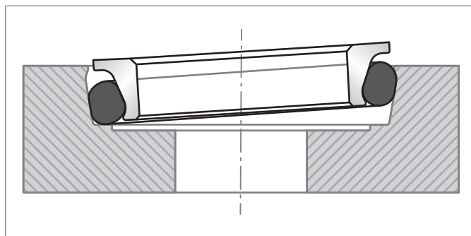
Figure 178: O形圈向底座滑动
