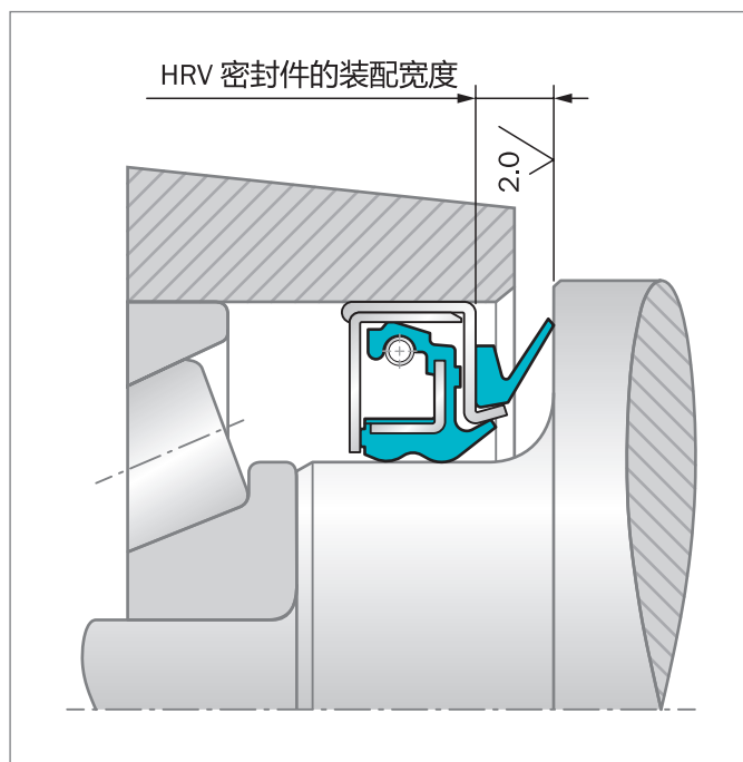
Figure 58: 带有 HRV 密封件的系统500
