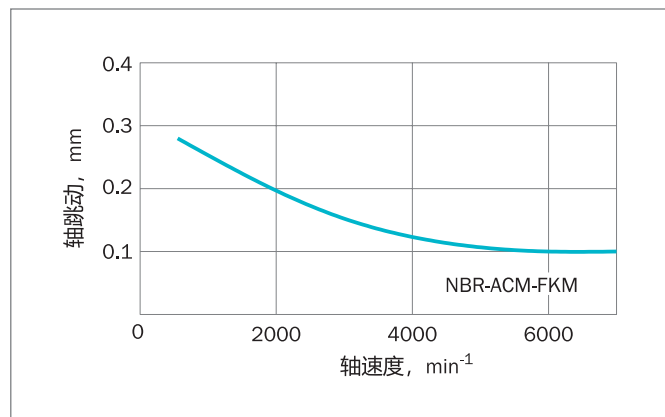
Figure 2: 轴跳动
